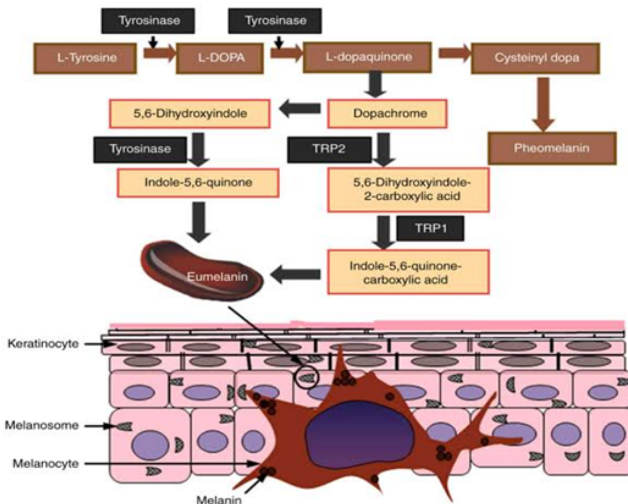
Figure 5. Inhibition process of tyrosinase [22]
