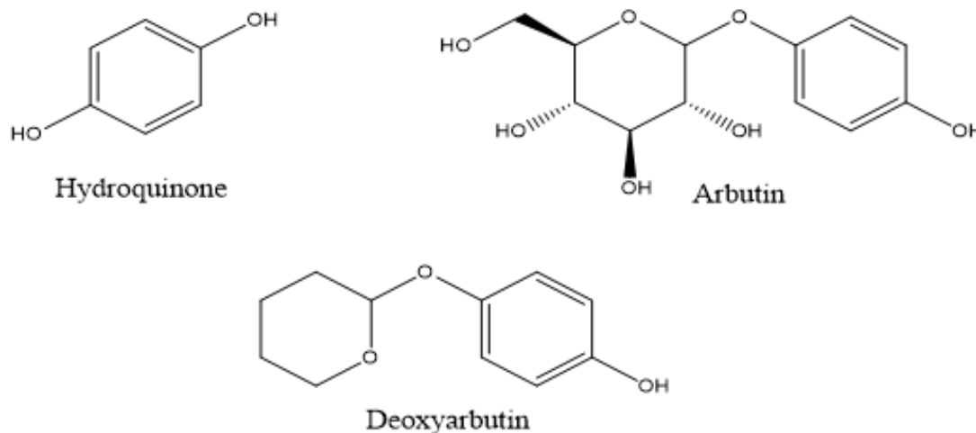
Figure 1. Structures of hydroquinone, arbutin and deoxyarbutin [12]
