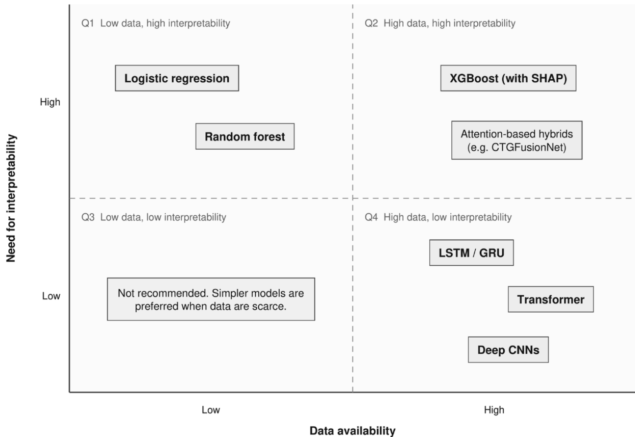
Figure 3: Conceptual model selection decision matrix for pregnancy prediction.
