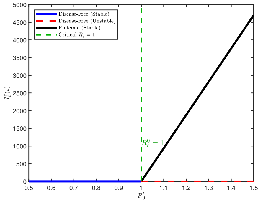
Figure 2: Bifurcation plot of the typhoid fever sub-model.
