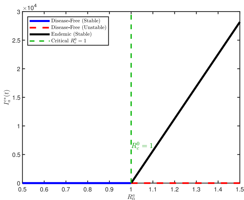
Figure 3: Bifurcation plot of amebiasis fever sub-model.
