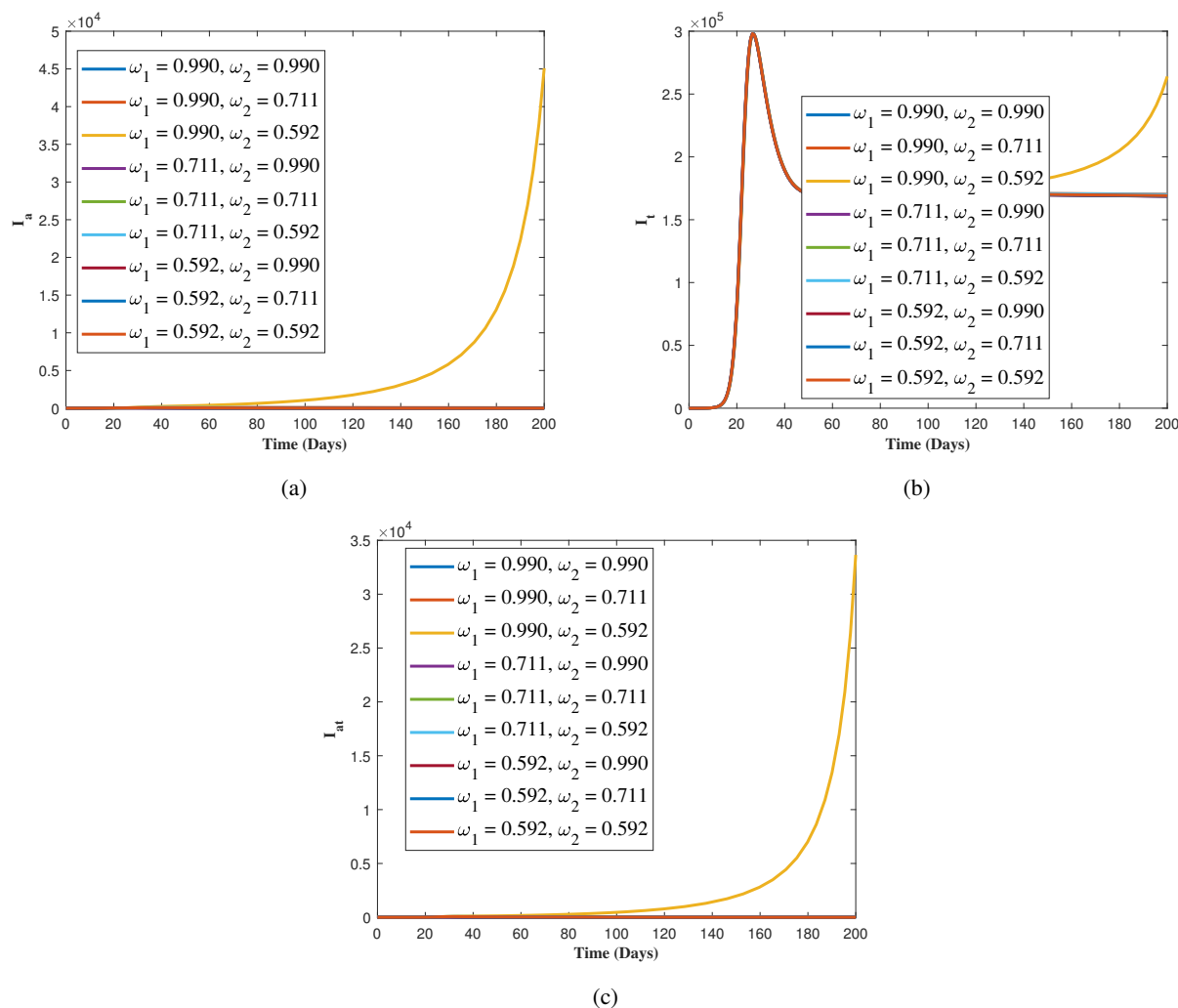
Figure 10: Varying values of \omega_1 and \omega_2 for (a) the infected and infectious population of amebiasis, ( I_a ), (b) the infected and infectious population of typhoid fever, ( I_t ), (c) co-infected and infectious population ( I_{at} ).
