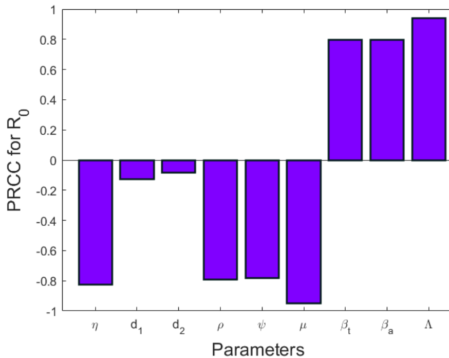
Figure 5: Partial rank correlation coefficient (PRCC) values illustrating the impact of parameters on R_0 .
