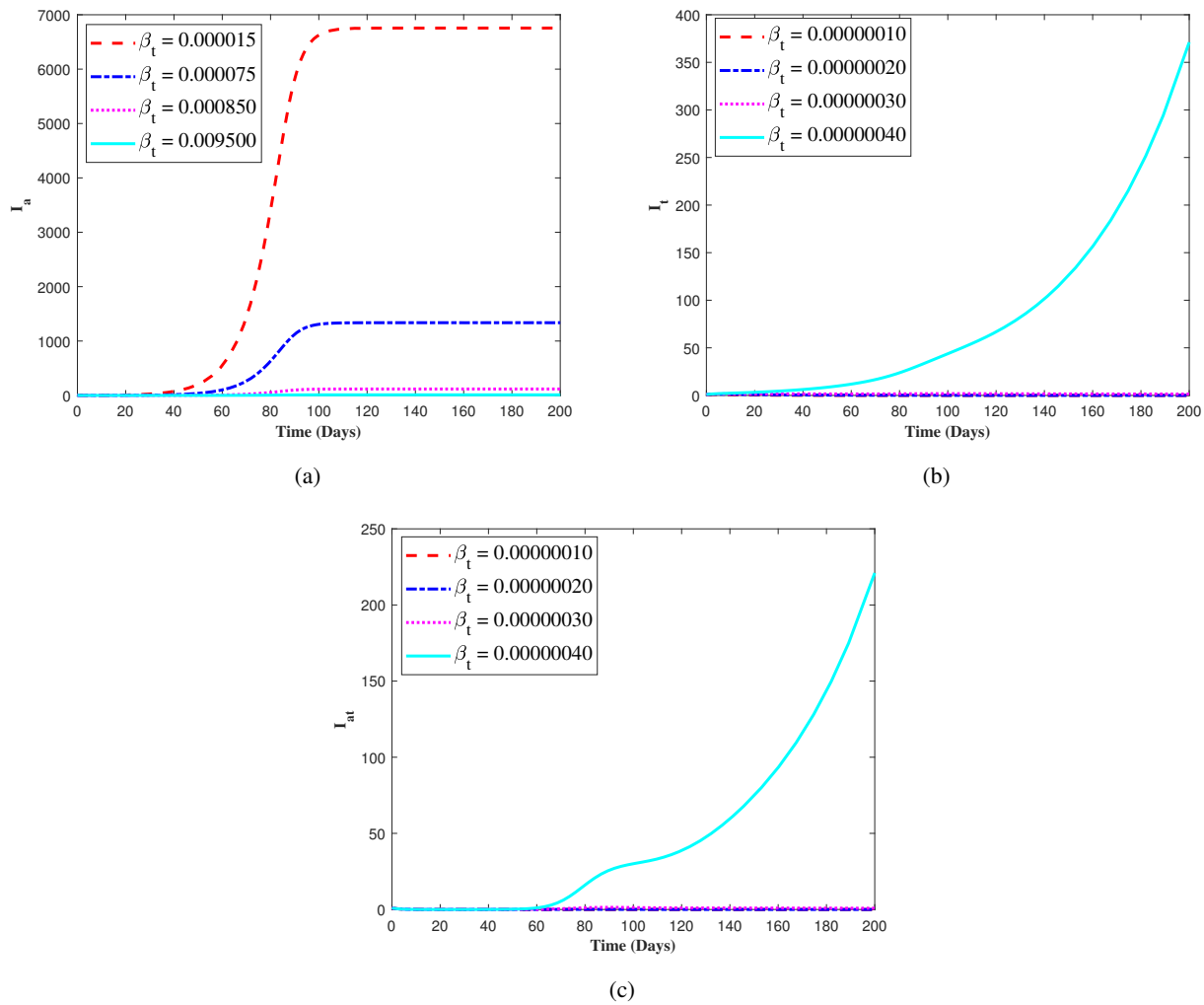
Figure 7: Varying values of \beta_t for (a) the infected and infectious population of amebiasis, ( I_a ), (b) the infected and infectious population of typhoid fever, ( I_t ), (c) co-infected and infectious population ( I_{at} ).
