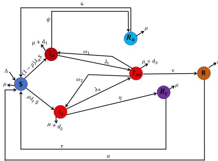
Figure 1: Typhoid fever–amebiasis co-dynamics flow diagram.
