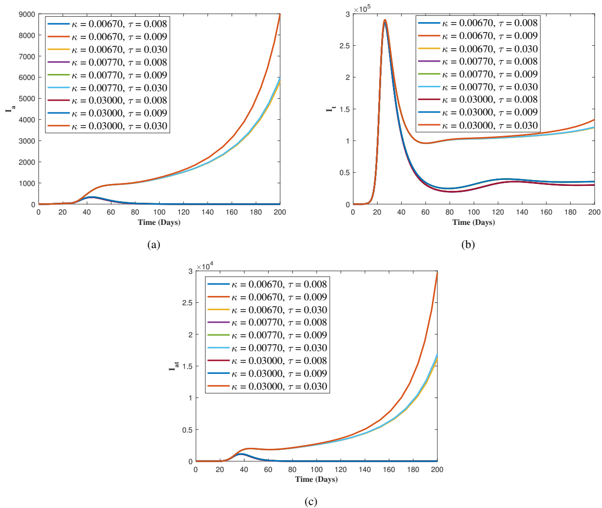
Figure 8: Varying values of \kappa and \tau for (a) the infected and infectious population of amebiasis, ( I_a ), (b) the infected and infectious population of typhoid fever, ( I_t ), (c) co-infected and infectious population ( I_{at} ).
