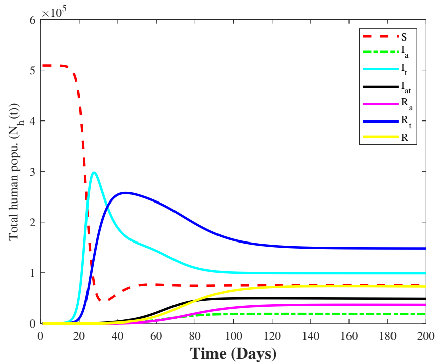
Figure 4: Plots of (a) S , I_a , I_t , I_{at} , R_a , R_t , and R .
