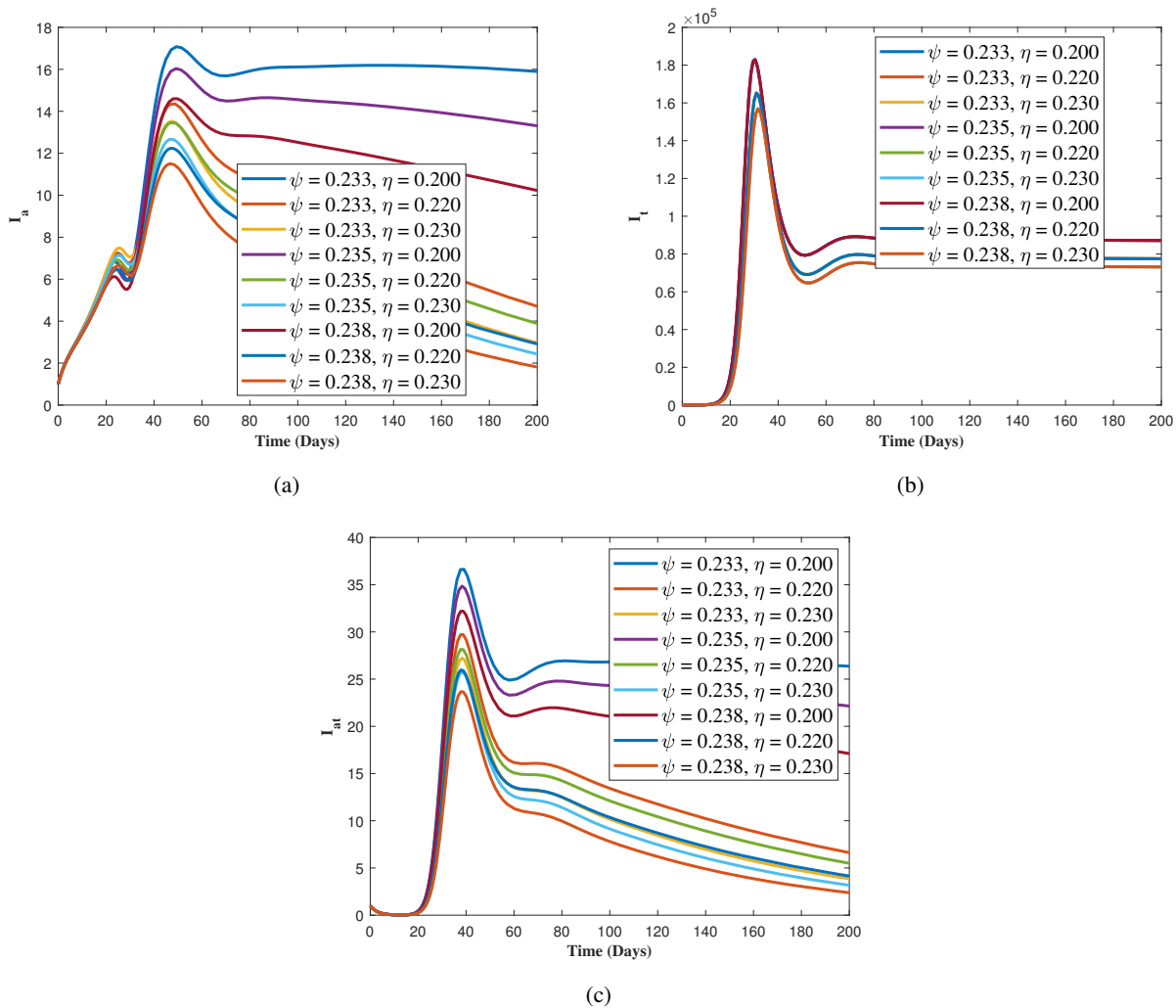
Figure 9: Varying values of \psi and \eta for (a) the infected and infectious population of amebiasis, ( I_a ), (b) the infected and infectious population of typhoid fever, ( I_t ), (c) co-infected and infectious population ( I_{at} ).
