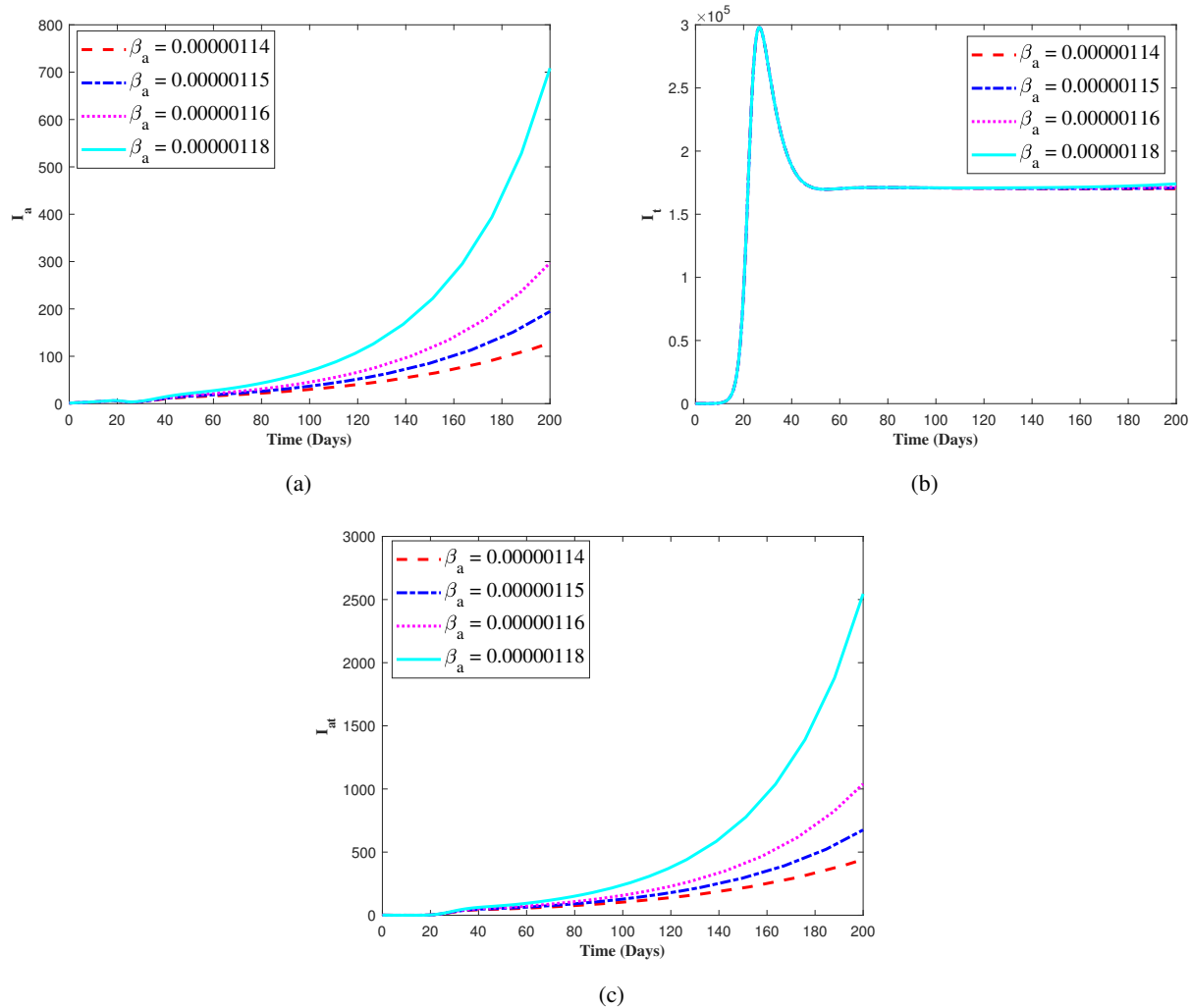
Figure 6: Varying values of \beta_a for (a) the infected and infectious population of amebiasis, ( I_a ), (b) the infected and infectious population of typhoid fever, ( I_t ), (c) co-infected and infectious population ( I_{at} ).
