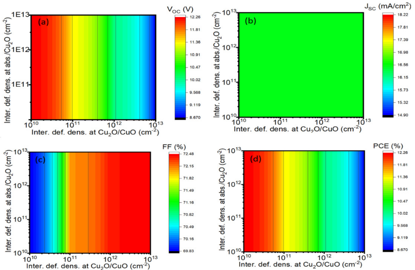
Figure 10: Contour mapping for varying (a) V_{OC} , (b) J_{SC} , (c) FF, and (d) PCE with defect densities at the absorber/ \text{Cu}_2\text{O} and \text{Cu}_2\text{O}/\text{CuO} interfaces.
