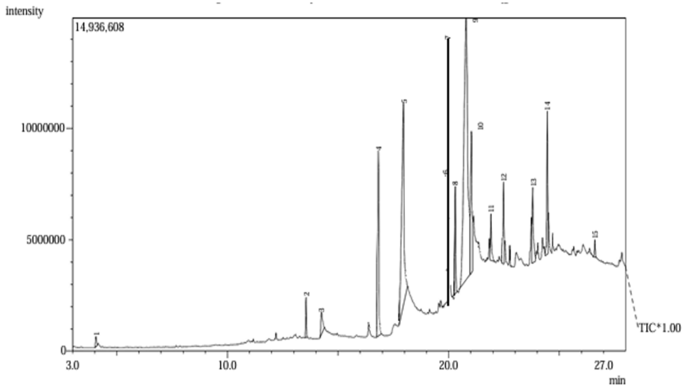
Figure 2: GC-MS chromatogram of aqueous extract of Ocimum gratissimum .
