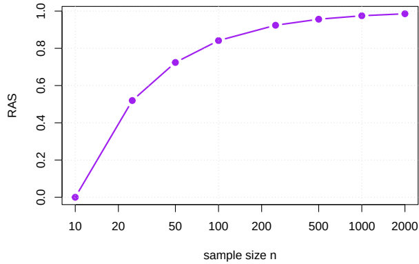
(c) Heavy-tailed t_3 .
