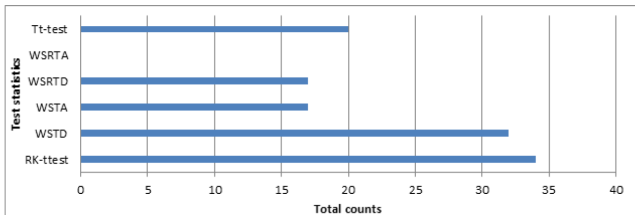
Figure 6. Bar chart indicating total times Type I error rates approximates to \alpha = 0.01
