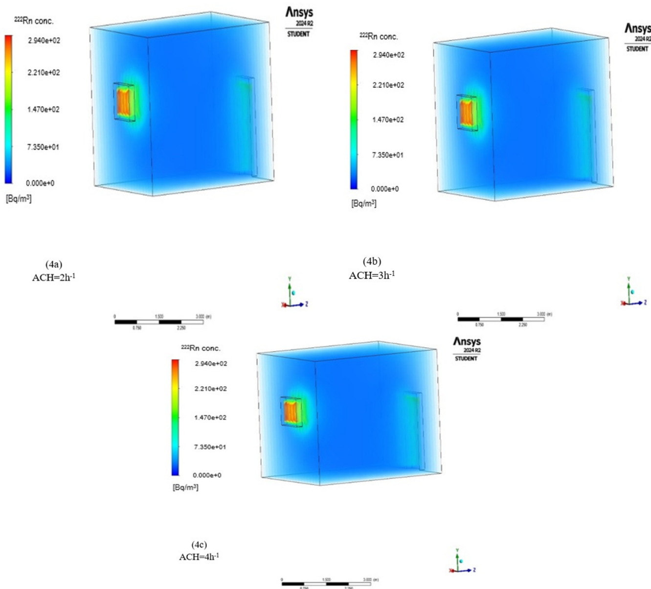
Figure 4: Radon concentration of 43.6 Bq/m 3 distribution at different ventilation rates in the test room model.
