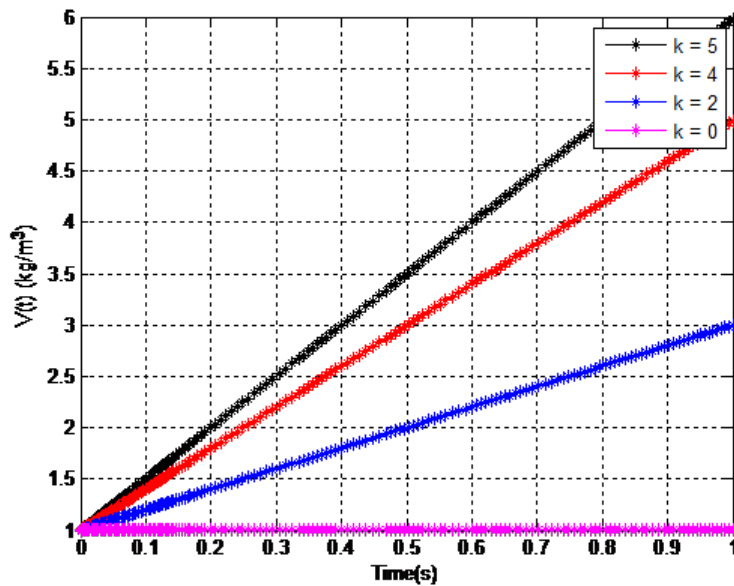
Figure 11. Variation of Water Droplet Number Density W(t) with Time for Zero formation of vapors, k .
