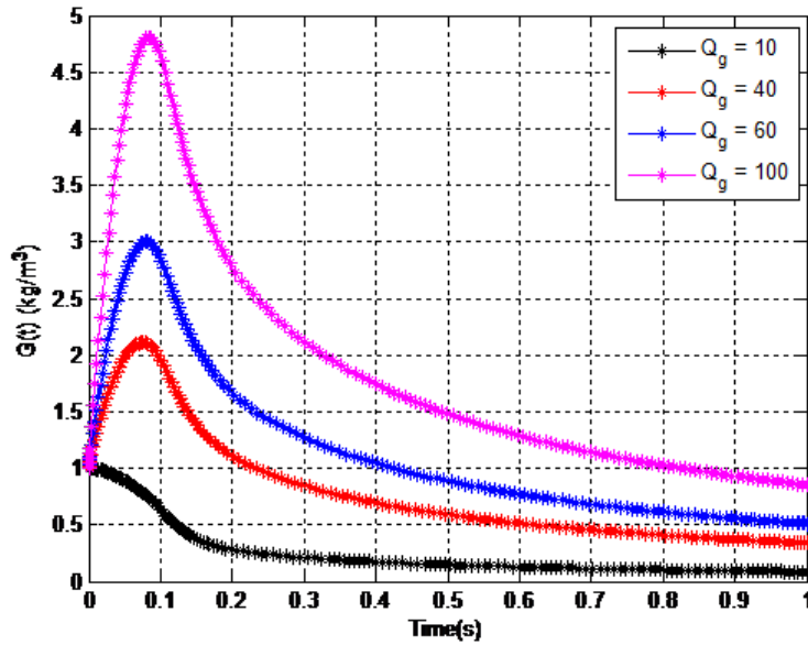
Figure 10. Variation of G with time t for different values of gaseous emission rates, Q_g .
