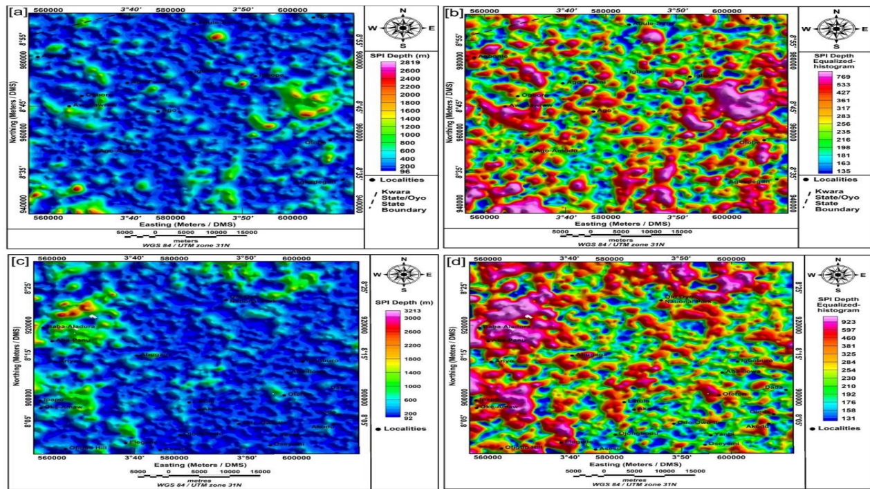
Figure 10: Source parameter imaging (SPI) maps of the study area presented using both linear (L) and equalized-histogram (H) color methods (a) Igboho sheet-L, (b) Igboho sheet-H, (c) Lechilaku sheet-L, (d) Lechilaku sheet-H.
