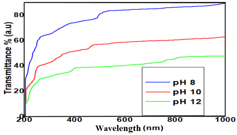
Figure 6. Transmittance spectral of ZnO nanoparticles at different pH.
