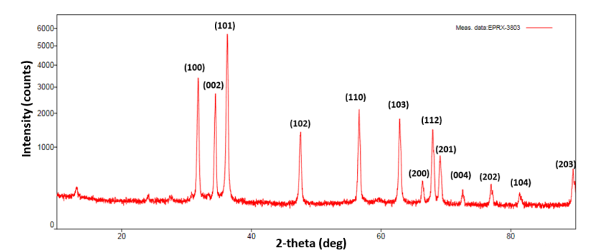
Figure 3. Diffraction pattern of ZnO NPs synthesized using pH 8.
