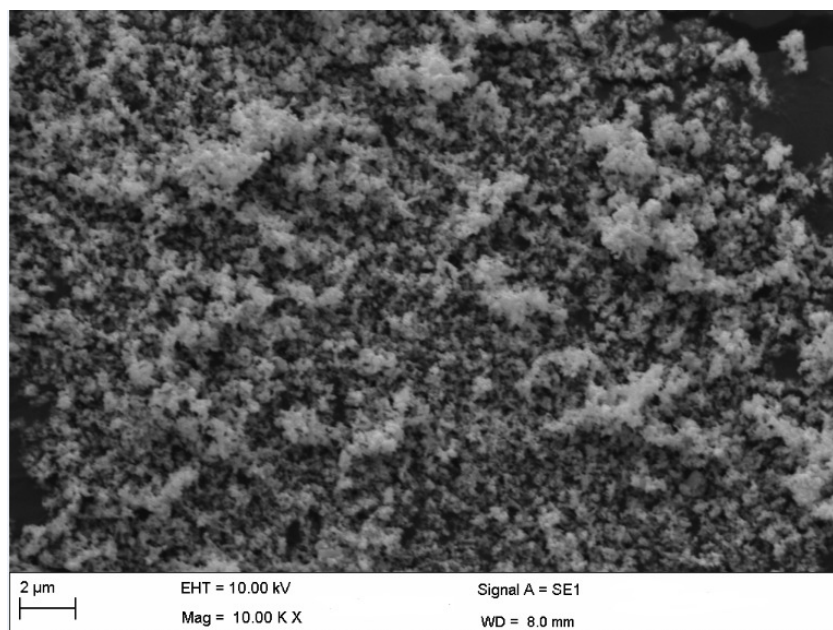
Figure 10. Surface morphology of ZnO nanoparticles at pH 10.
