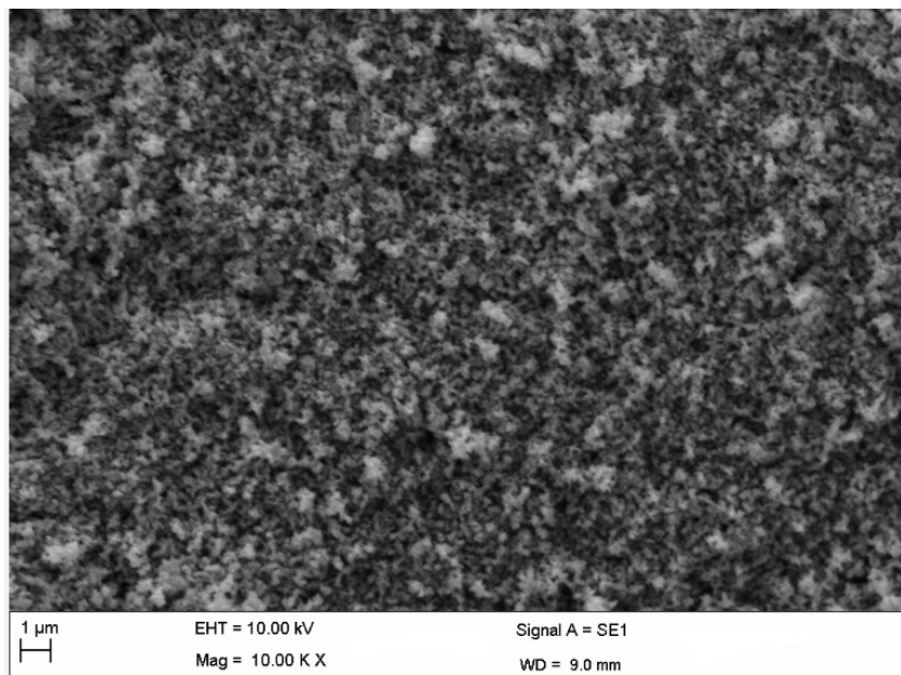
Figure 9. Surface morphology of ZnO nanoparticles at pH 12.
