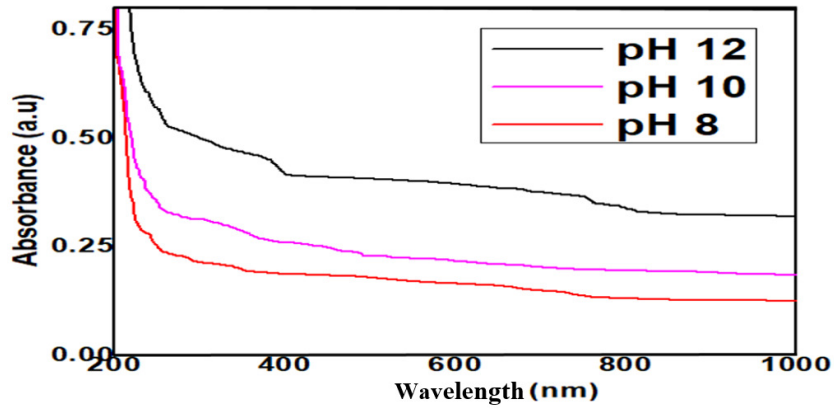
Figure 8. Absorption spectral of ZnO NPs at different pH.
