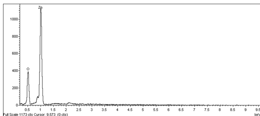
Figure 2. Spectral showing the Energy Dispersive X-ray Spectroscopy of ZnO sample.
