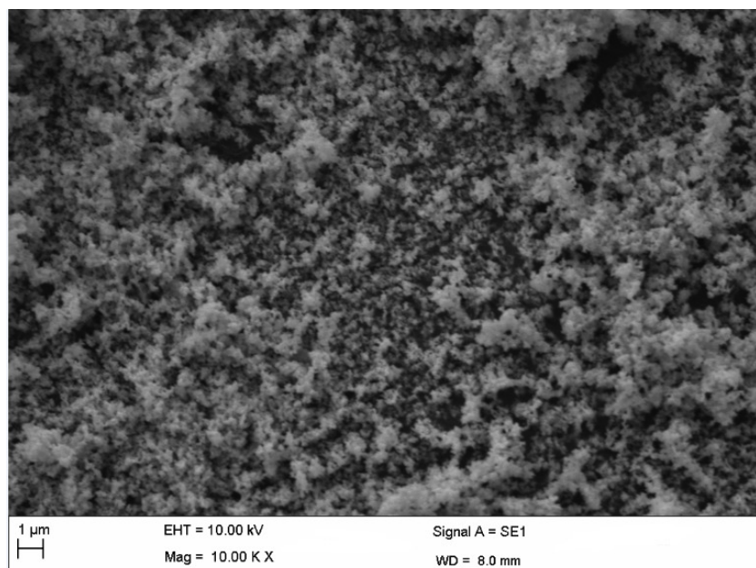
Figure 11. Surface morphology of ZnO nanoparticles at pH 8.
