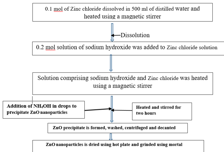
Figure 1. Schematic diagram of experimental procedure of zinc oxide nanoparticles.
