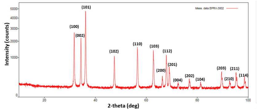
Figure 5. Diffraction pattern of ZnO NPs synthesized using pH 12.
