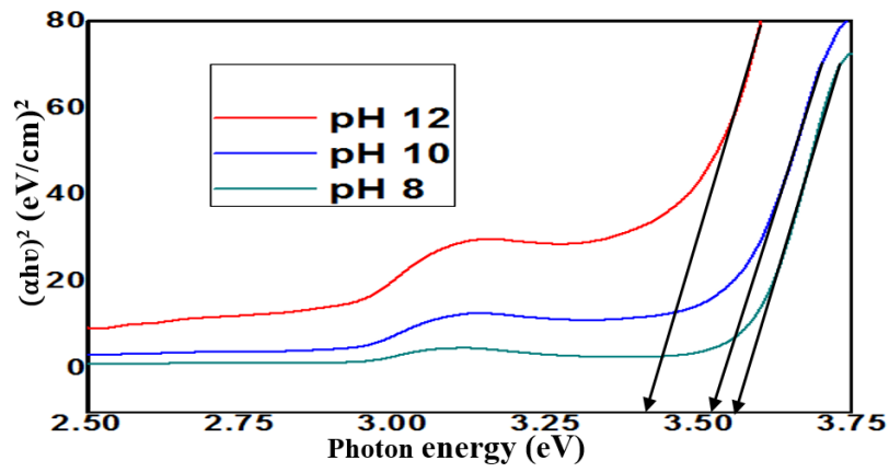
Figure 7. Optical energy band gap of ZnO NPs at different pH.
