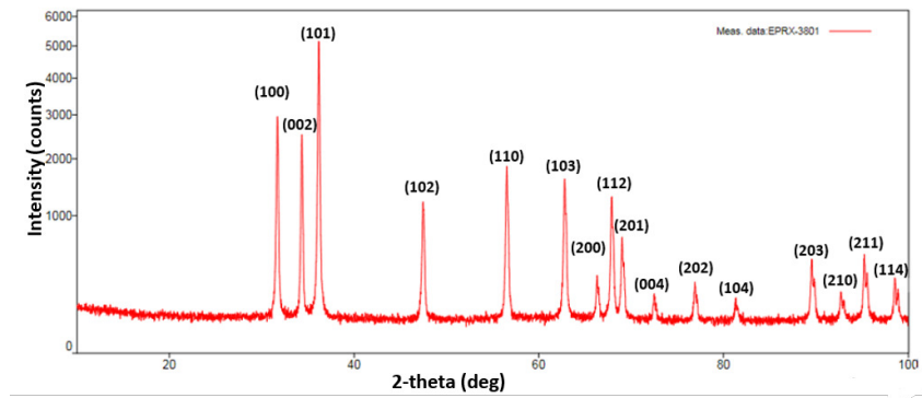
Figure 4. Diffraction pattern of ZnO NPs synthesized using pH 10.
