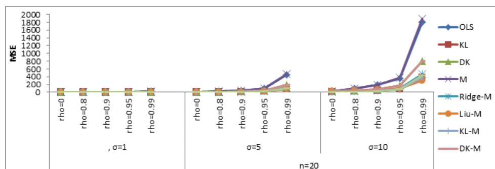
Figure 1. Graph of estimated MSEs of all the estimators when there is no outlier at all levels of multicollinearity and sample size ( n ) = 20.
